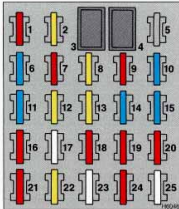
Left Side Fuse Panel
